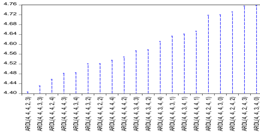
Akaike Information Criteria (top 20 models)
